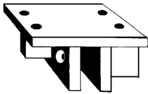
RP: for steel girder formwork with angle profiles and special steel profiles
